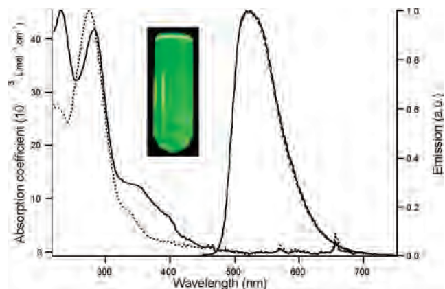
Figure 5. Absorption (left) and emission (right) of N984 (dotted lines) and N984b (full lines) in solution in acetonitrile. The insert shows a photo of the 10^{-5} M N984b solution emission exhibiting a very strong green color when excited at 365 nm.
