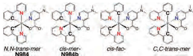
Figure 3. Structure of possible isomers of N984 . Nitrogen atoms are highlighted for clarity.
